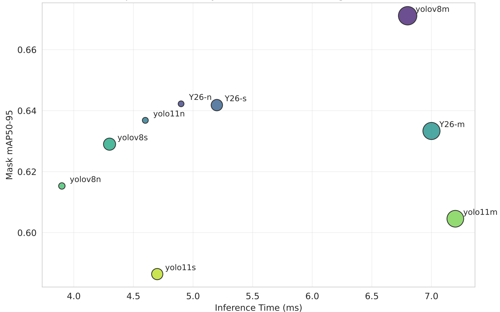
Speed vs Accuracy Tradeoff — YOLO26 Segmentation
