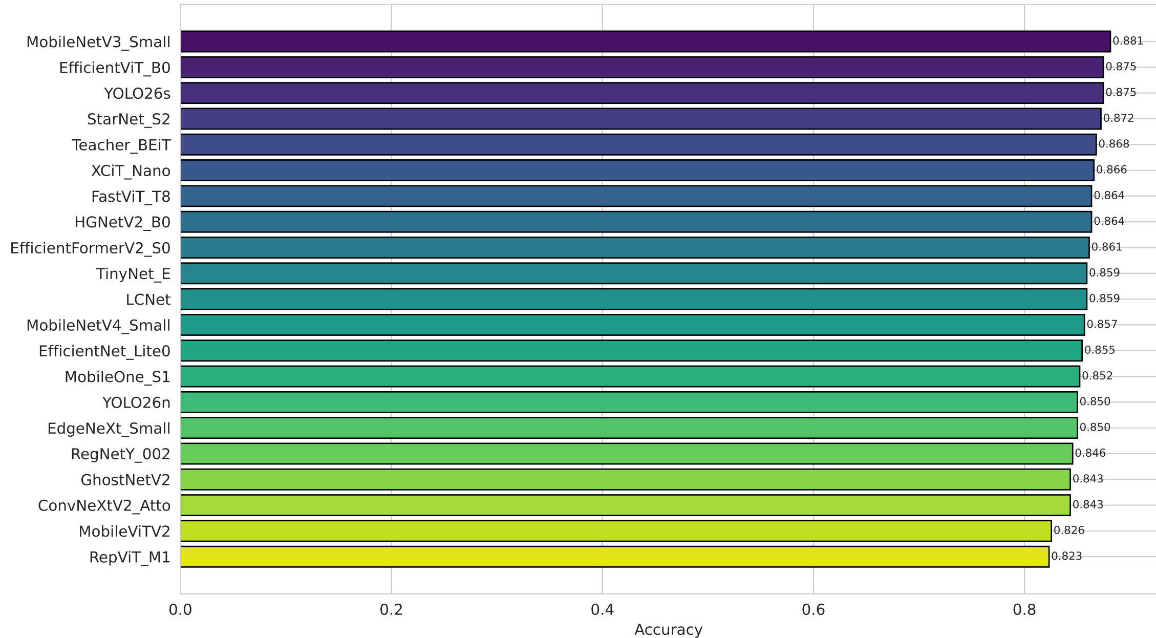
Cat Sound — Model Comparison
