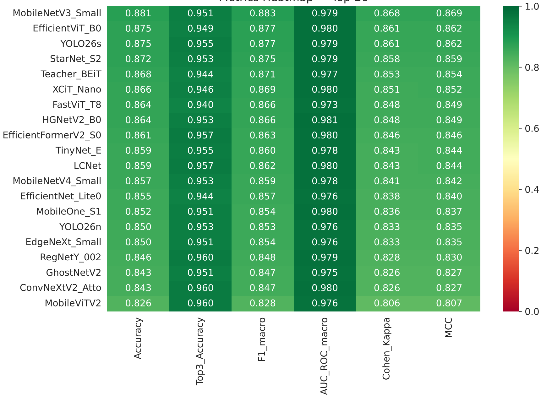
Metrics Heatmap — Top-20
