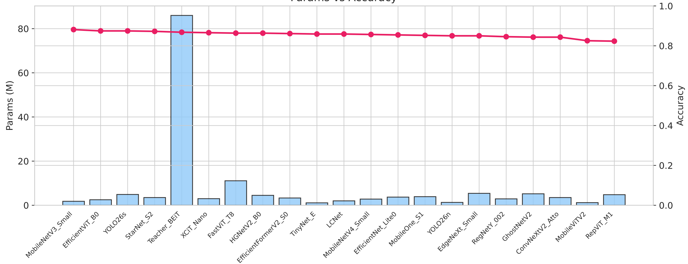
Params vs Accuracy
