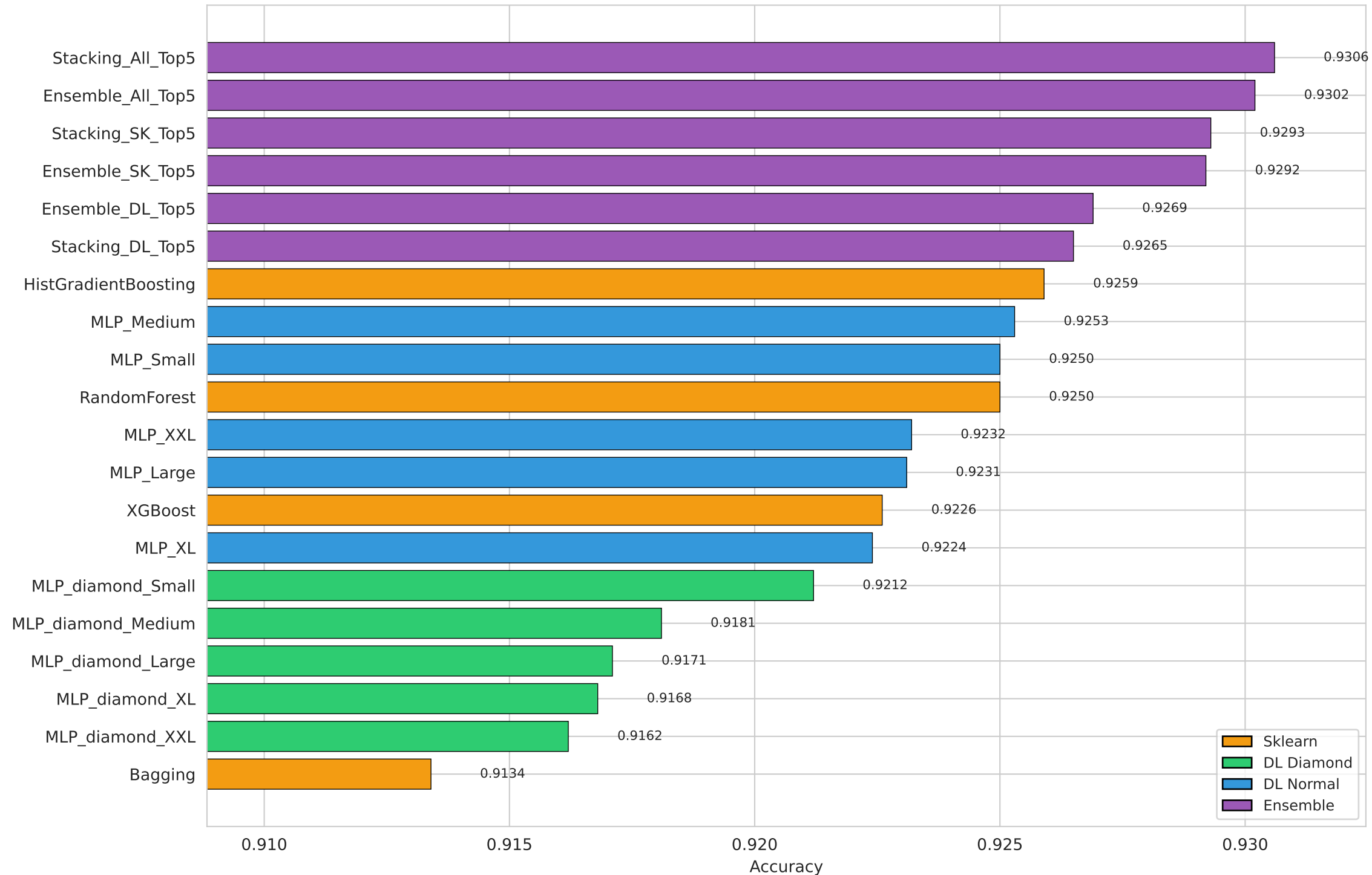
Top-20 Models by Accuracy
