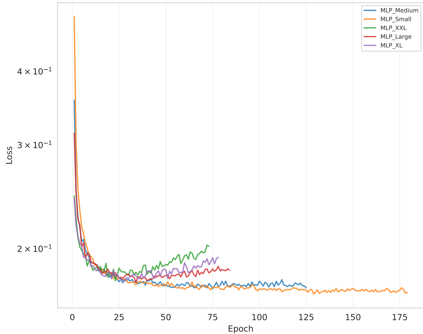
Validation Loss (Top-5 DL)
