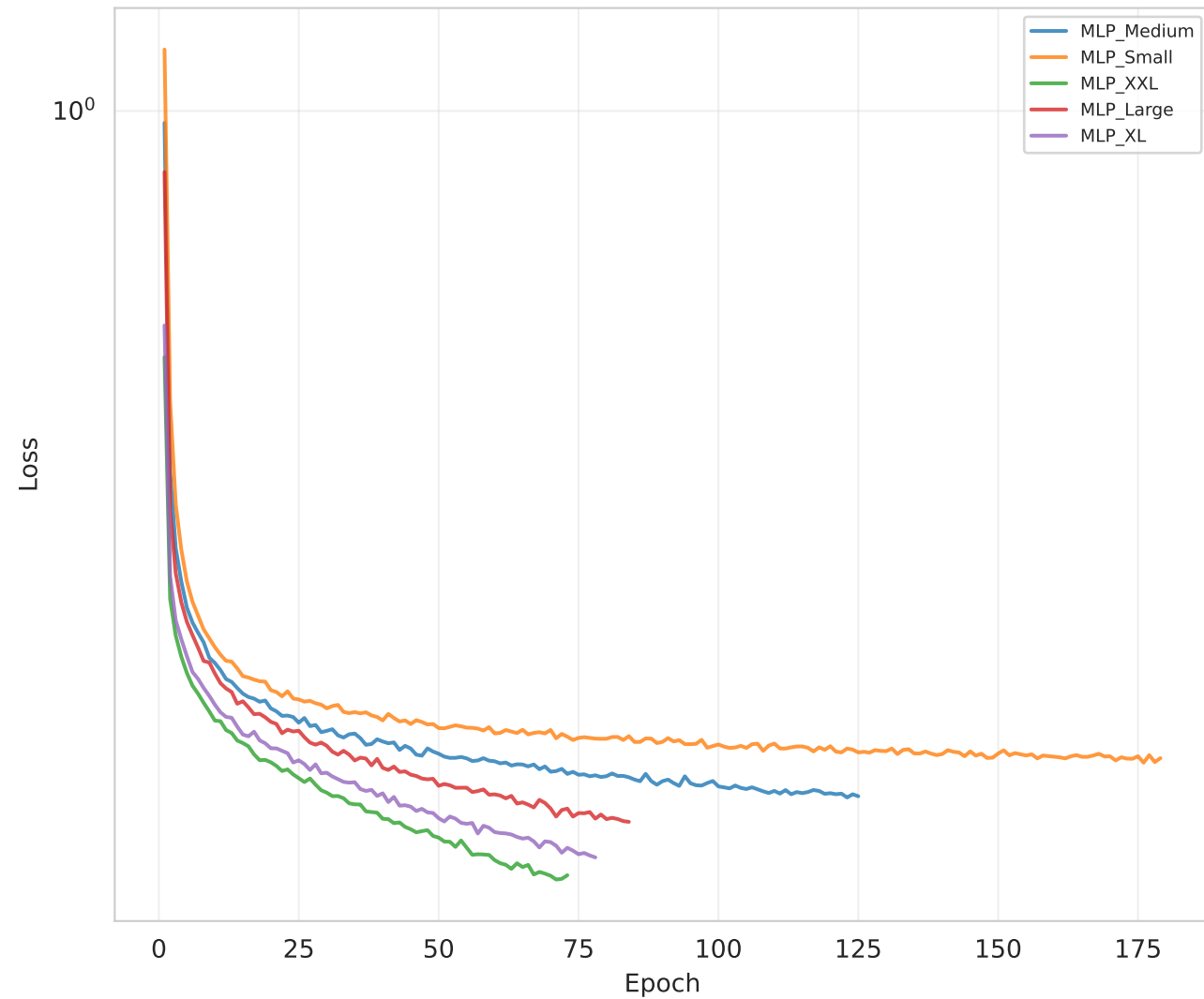
Training Loss (Top-5 DL)
