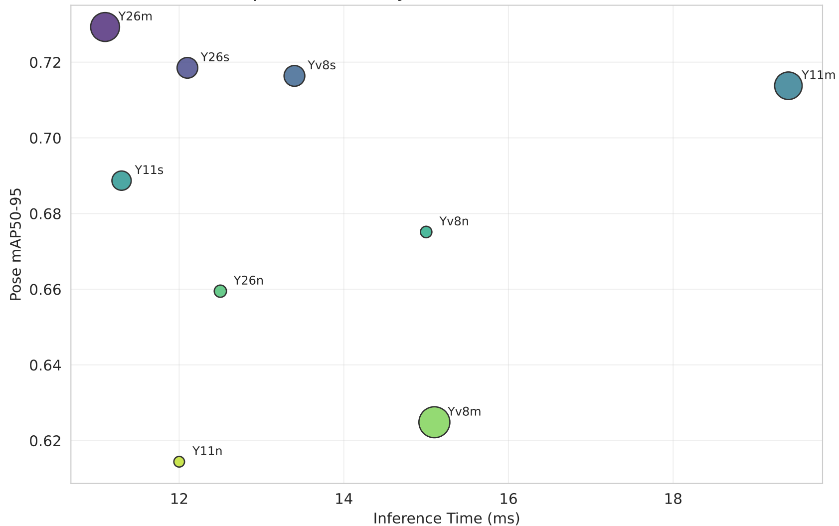
Speed vs Accuracy — Cat Landmark Detection
