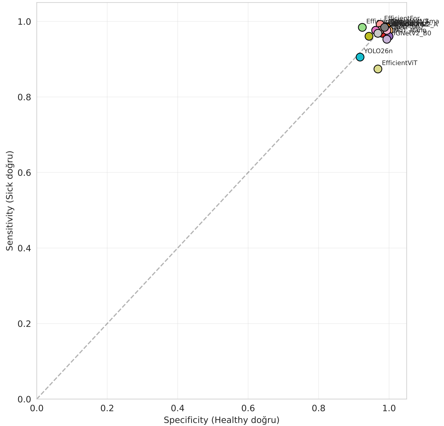
Sensitivity vs Specificity Tradeoff
