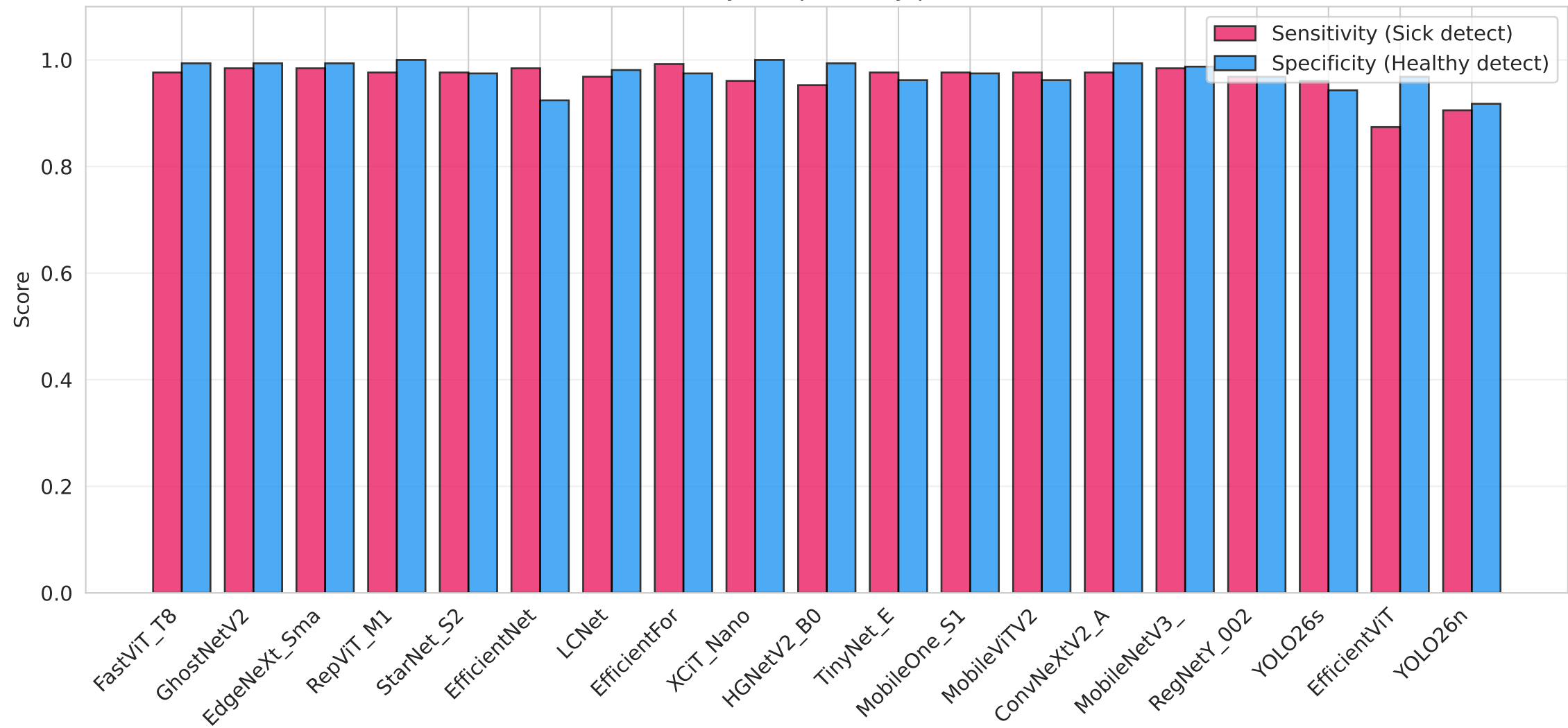
Sensitivity vs Specificity per Model
