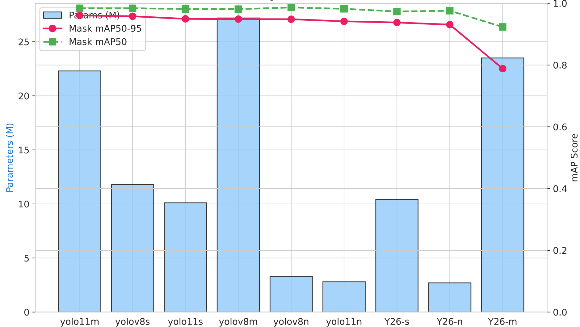
Model Size vs Segmentation Performance
