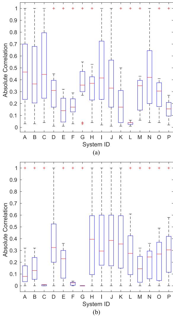
Fig. 7. Boxplot of absolute correlations across countermeasures. (a) Known attacks. (b) Unknown attacks.
