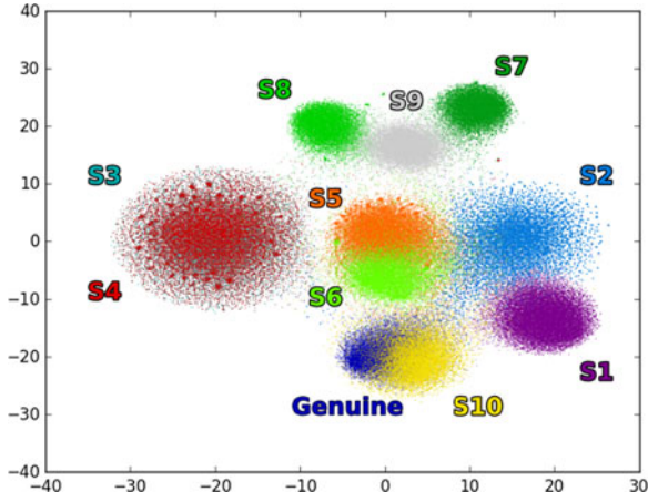
Fig. 2. Visualization of differences between genuine and spoofed speech in the ASVspoof 2015 database. Two-dimensional data were produced using a t-distributed stochastic neighbor embedding (t-SNE) algorithm applied to high-dimensional i-vector representations of each utterance.
