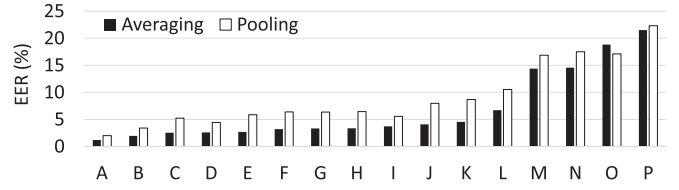
Fig. 6. Comparison of primary submitted systems in terms of EERs computed by averaging (as in ASVspoof evaluation plan) and pooling.
