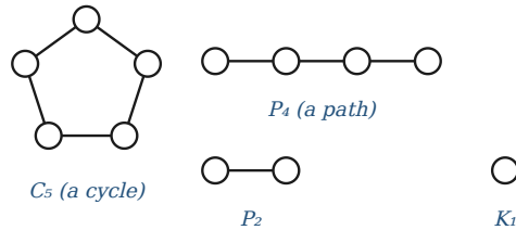
A typical graph with \Delta(G) \leq 2 : components are paths (including isolated vertices) and cycles. Here \Delta(G) = 2 and \delta(G) = 0 .
