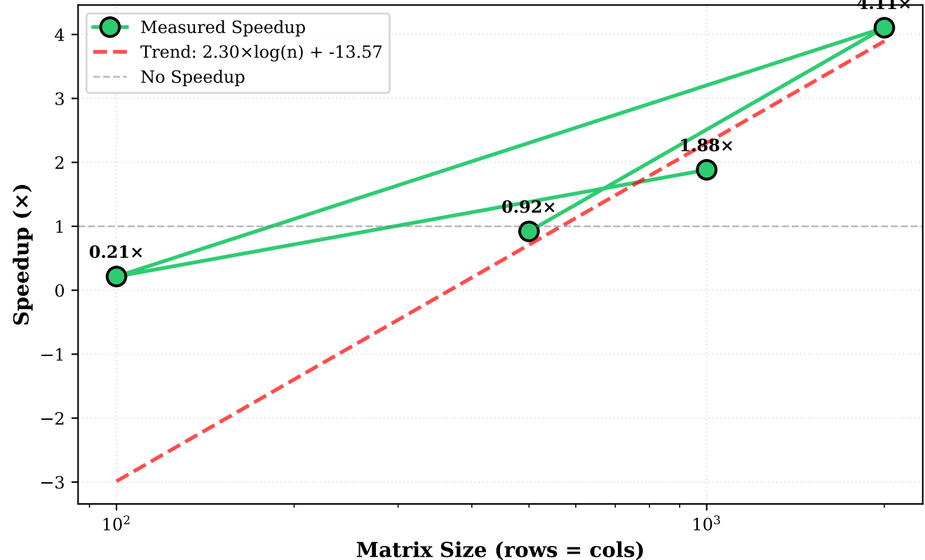
(b) Scaling Analysis: Speedup vs Matrix Size
