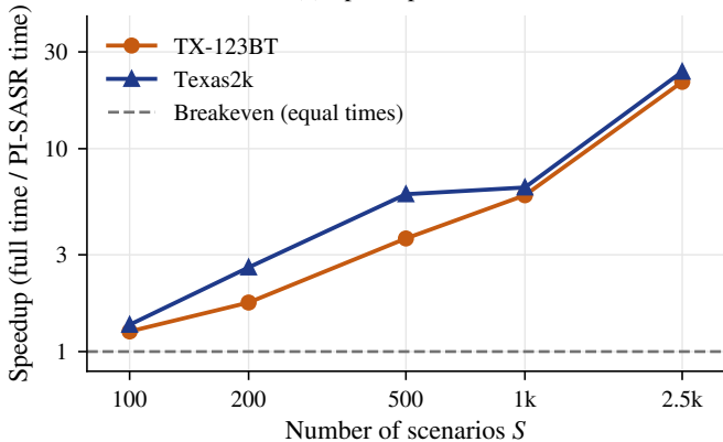
(a) Speedup versus S
