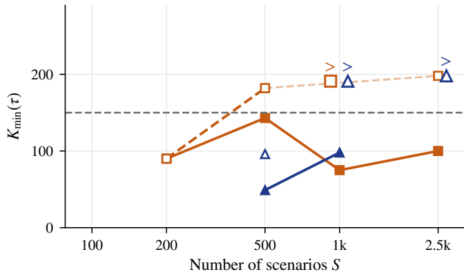
(b) Minimum active-set size K_{\min}(\tau)
