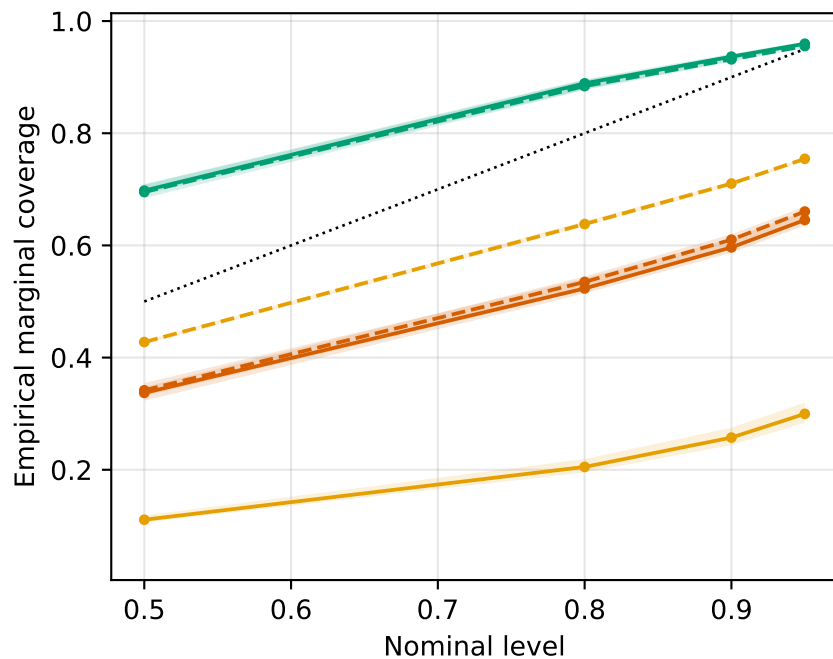
ID test — uncalibrated bands
