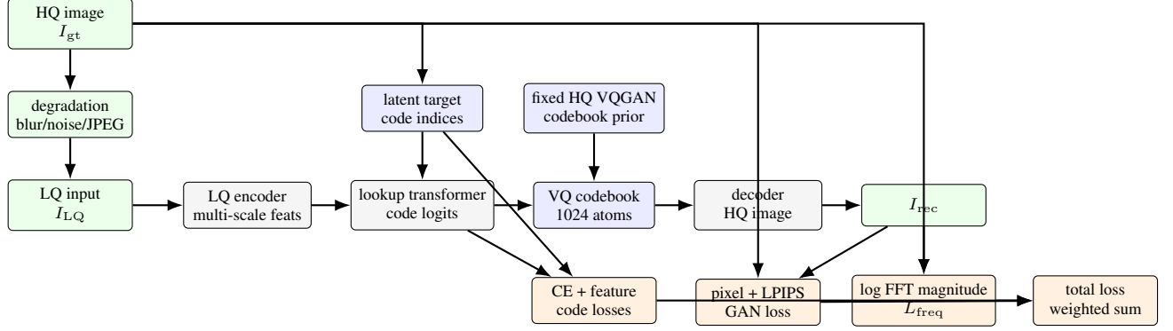
Figure 1: Detailed spectral-aware CodeFormer training pipeline. Degraded inputs are encoded and mapped to high-quality code indices by the lookup transformer. The VQ codebook and decoder reconstruct the image, while pixel, perceptual, adversarial, code prediction, and log-Fourier losses supervise complementary properties.
