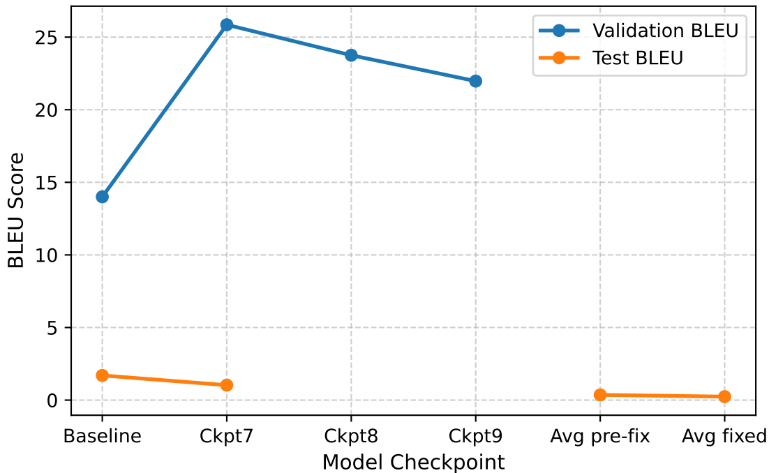
Validation vs. Test BLEU Across Checkpoints
