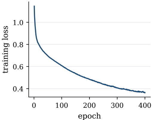
MLP ( \hat{m}(Y_{t-1}), L_2 )
