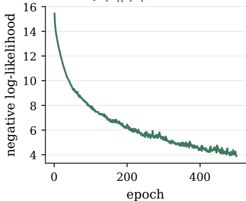
MDN ( \hat{f}_{X_{t-1}|Y_{t-1}} )
