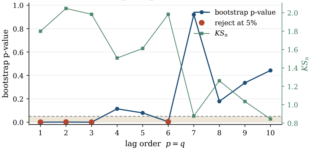
CSI 300, 2021-2024, P_t \rightarrow V_t
