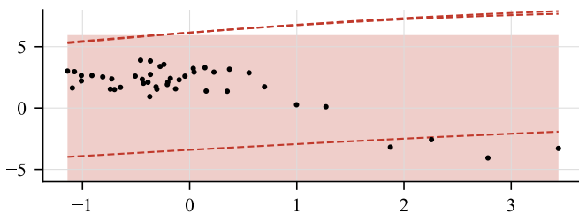
(c) Gaussian kernel: \kappa = 0.1
