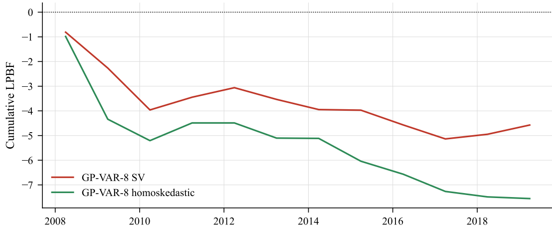
Cumulative joint LPBF vs. BVAR-8, h = 1
