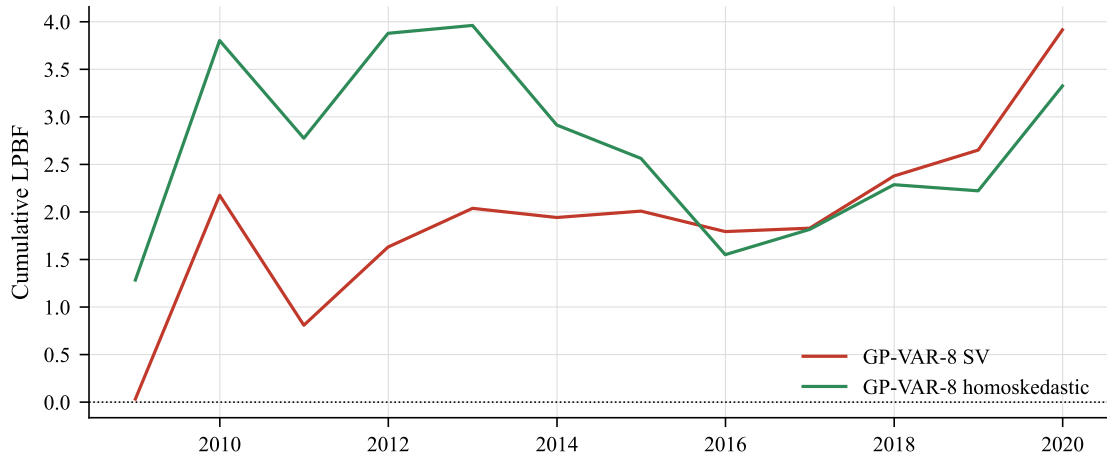
Cumulative joint LPBF vs. BVAR-8, h = 4
