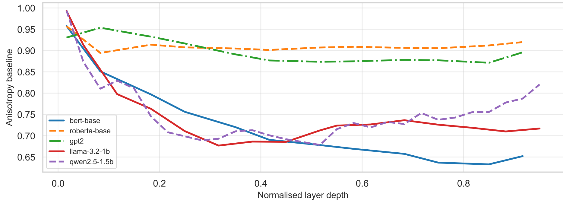
Anisotropy profile across models
