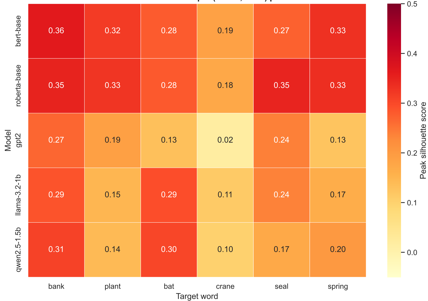
Peak silhouette score per (model, word) pair
