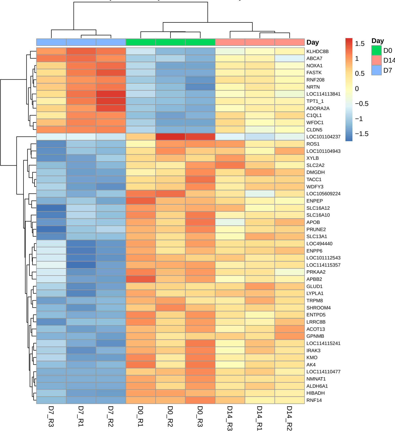
Top 50 DEGs (scaled VST counts)
