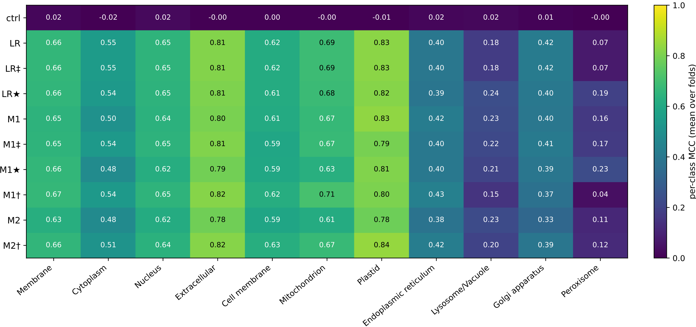
Cross-validated per-class MCC by model (whole-cell, 11 compartments)
