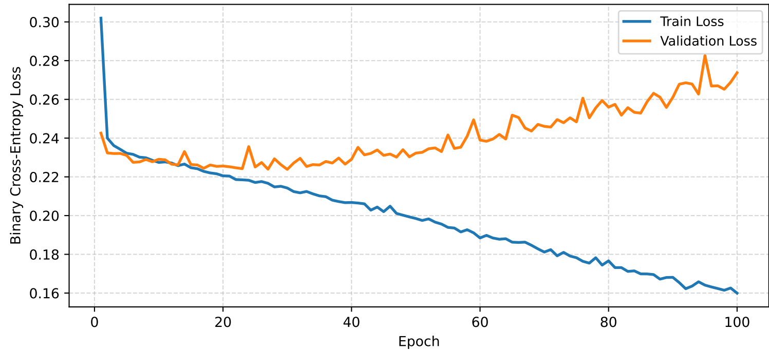
Sub-Nuclear 2H-MLP Training & Validation Loss
