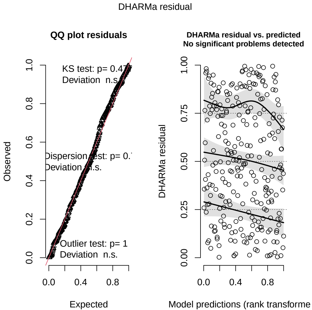
Figure 2: DHARMA Residuals diagnostics for the selected logistic regression model predicting bird nest occurrence from tree height, acacia ant species, and their interaction. The left panel shows a QQ plot comparing simulated and expected residual distributions. The right displays DHARMA residuals plotted against model predictions.
