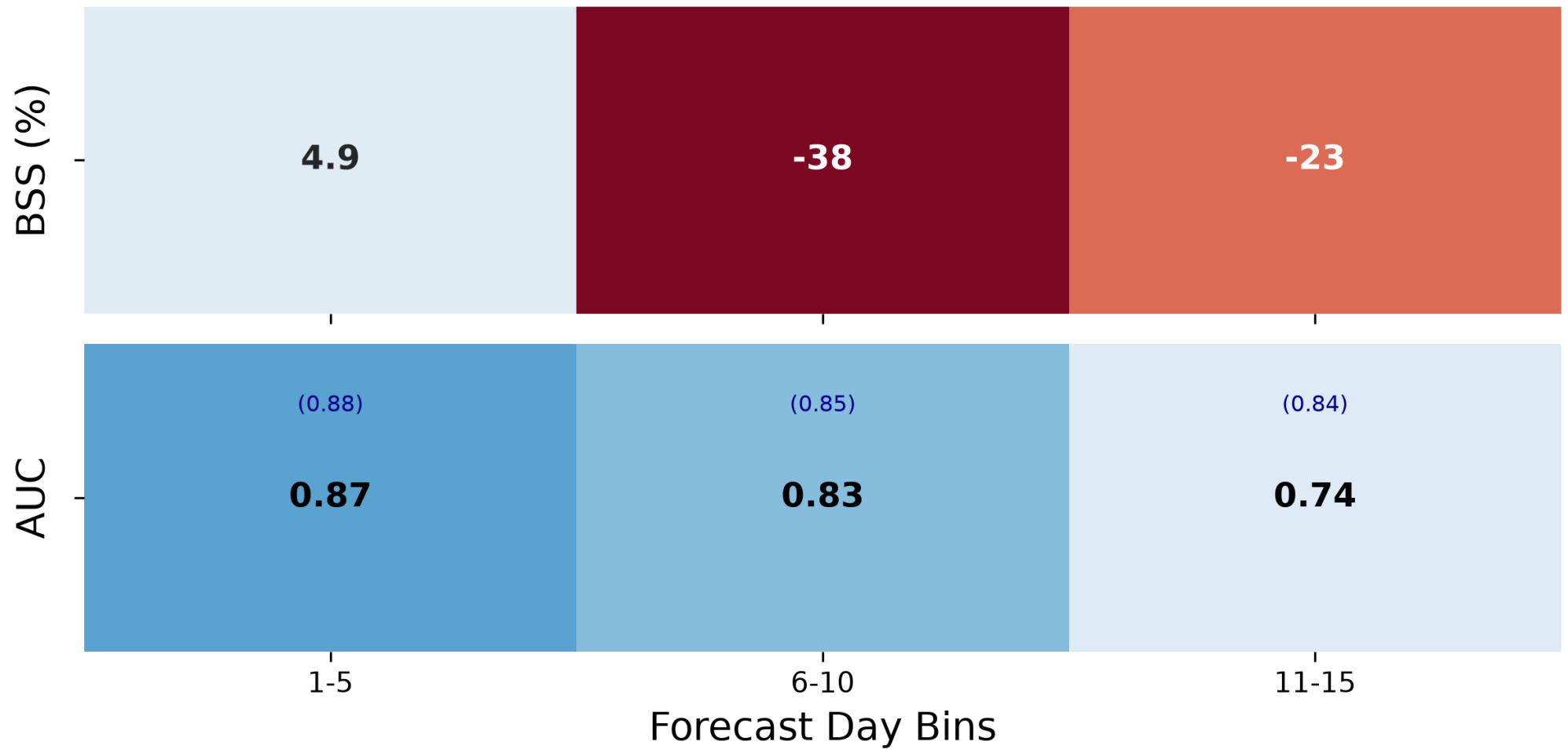
Skill Scores Heatmap - GenCast - Days 1-15
