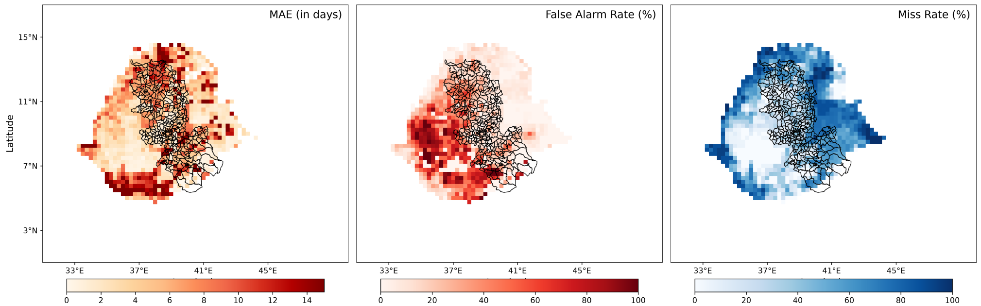
Spatial Metrics - AIFS - Days 1-15
