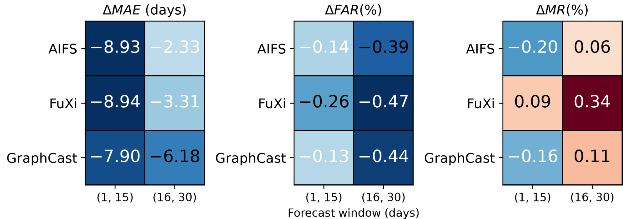
Panel Portrait: MAE / FAR / MR - AIFS (30-day)
