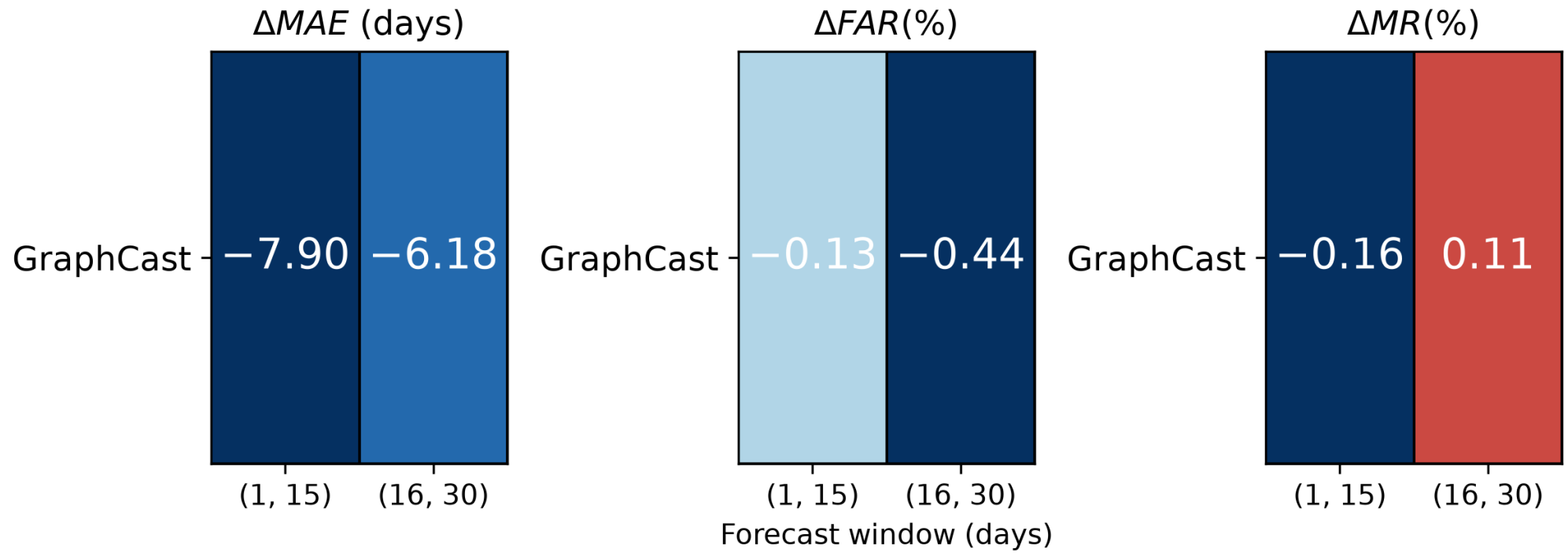
Panel Portrait MAE / FAR / MR - GraphCast - 30-day
