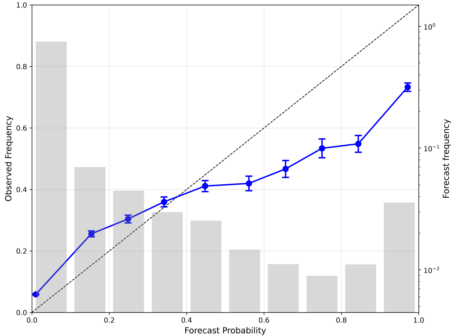
Reliability Diagram - GenCast - Days 1-15
