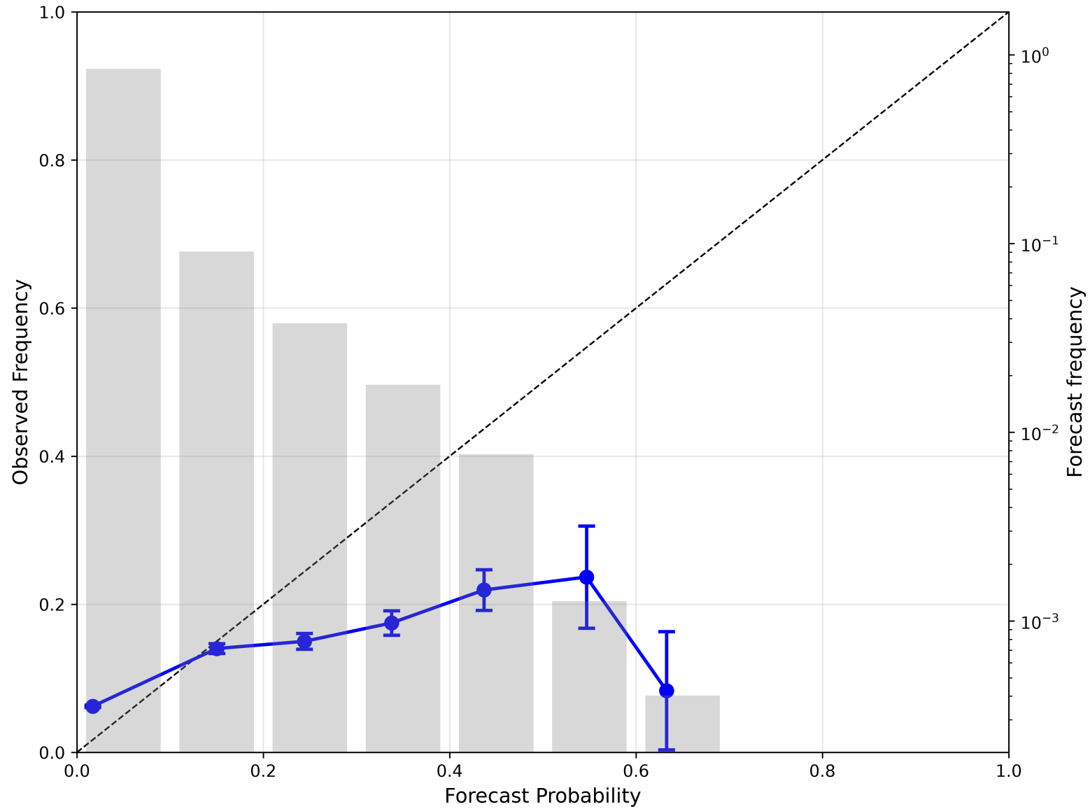
Reliability Diagram - GenCast - Days 16-30
