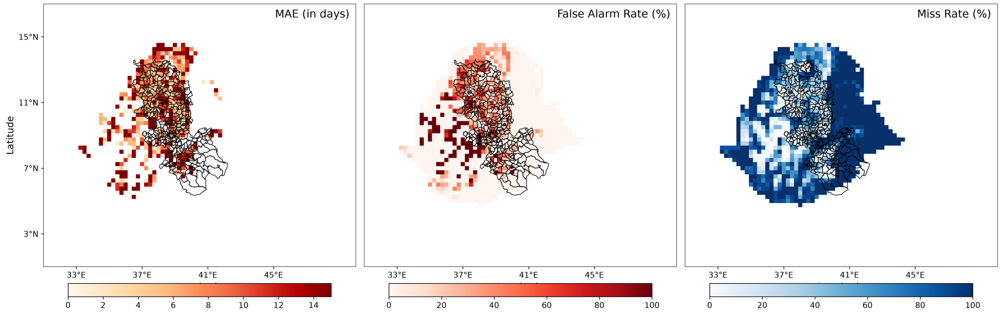
Spatial Metrics - FuXi - Days 16-30
