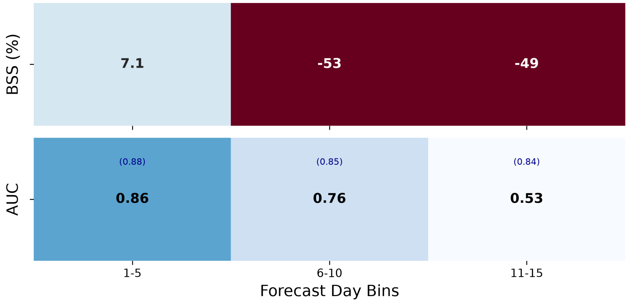
Skill Scores Heatmap (8)
