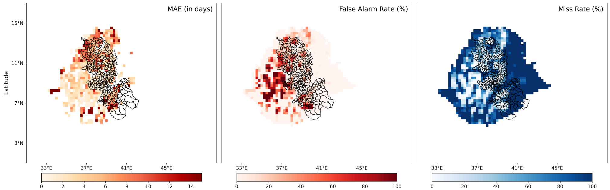
Spatial Metrics - FuXi - Days 1-15
