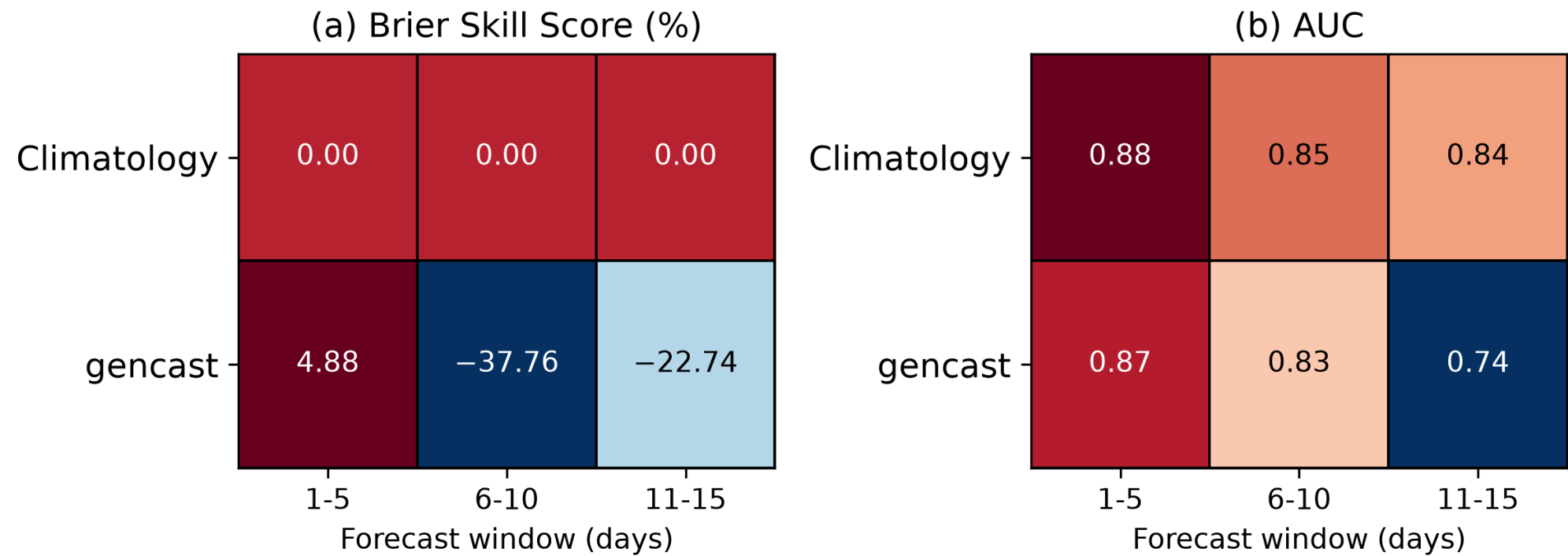
Panel Portrait - Days 1-15
