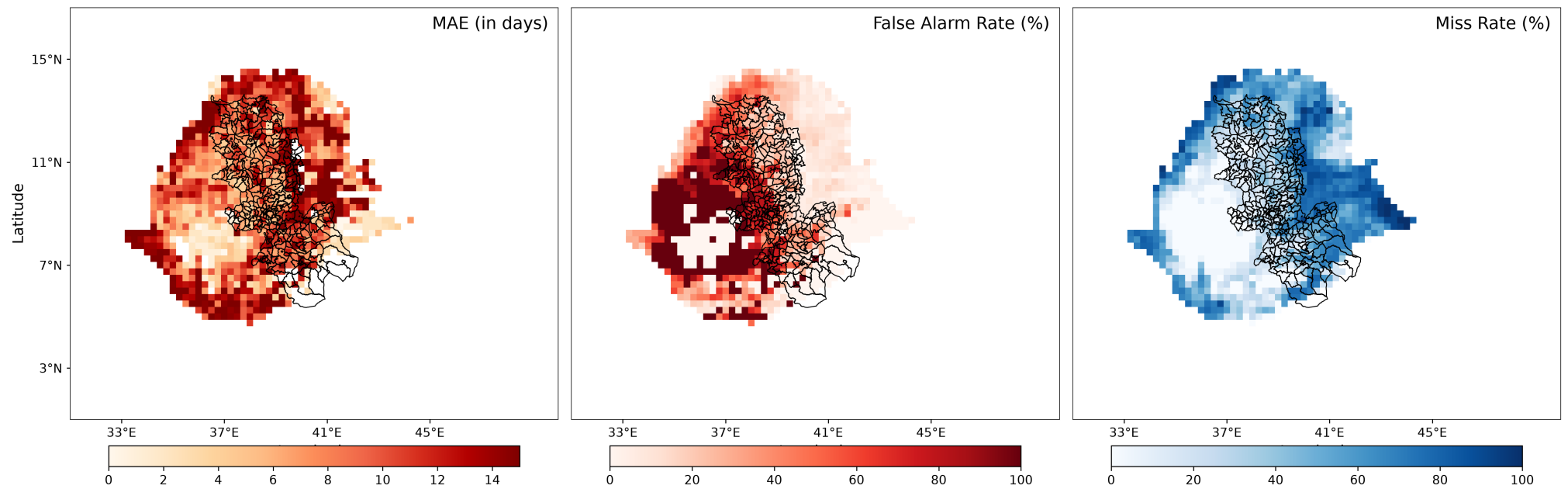
Spatial Metrics - AIFS - Days 16-30
