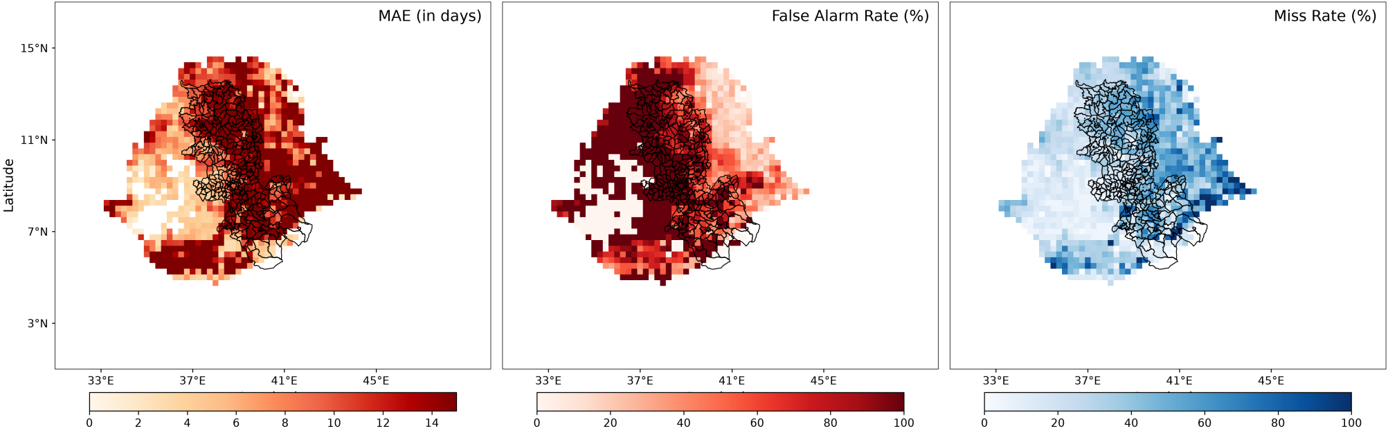
Spatial Metrics: Climatology (Days 16-30)
