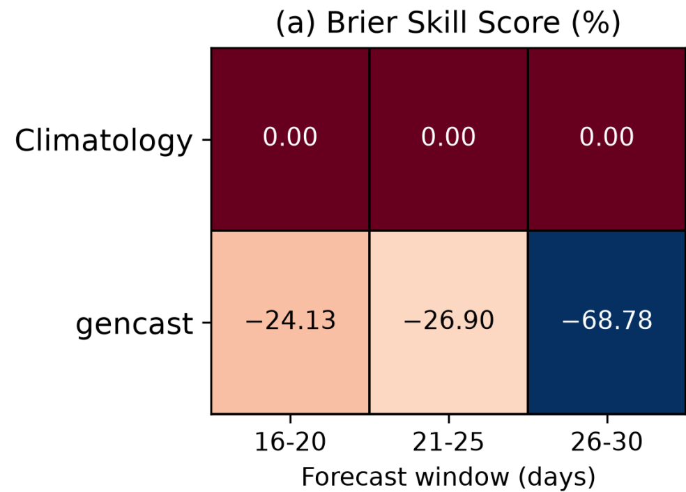
Panel Portrait - Days 16-30
