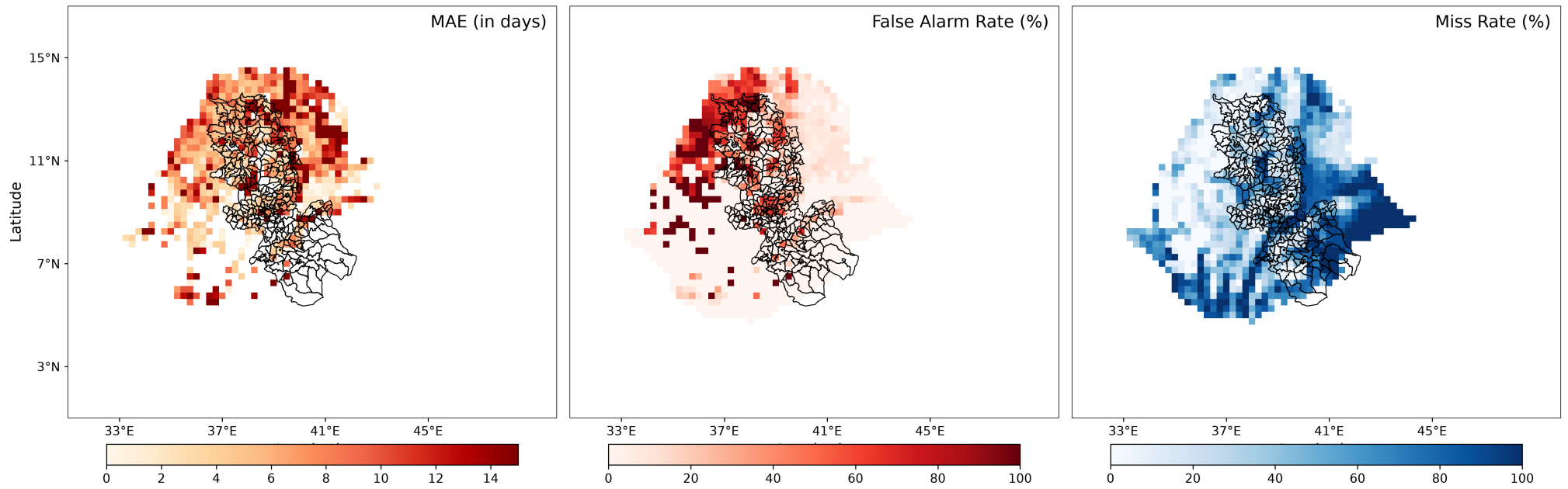
Spatial Metrics - GraphCast - Days 16-30
