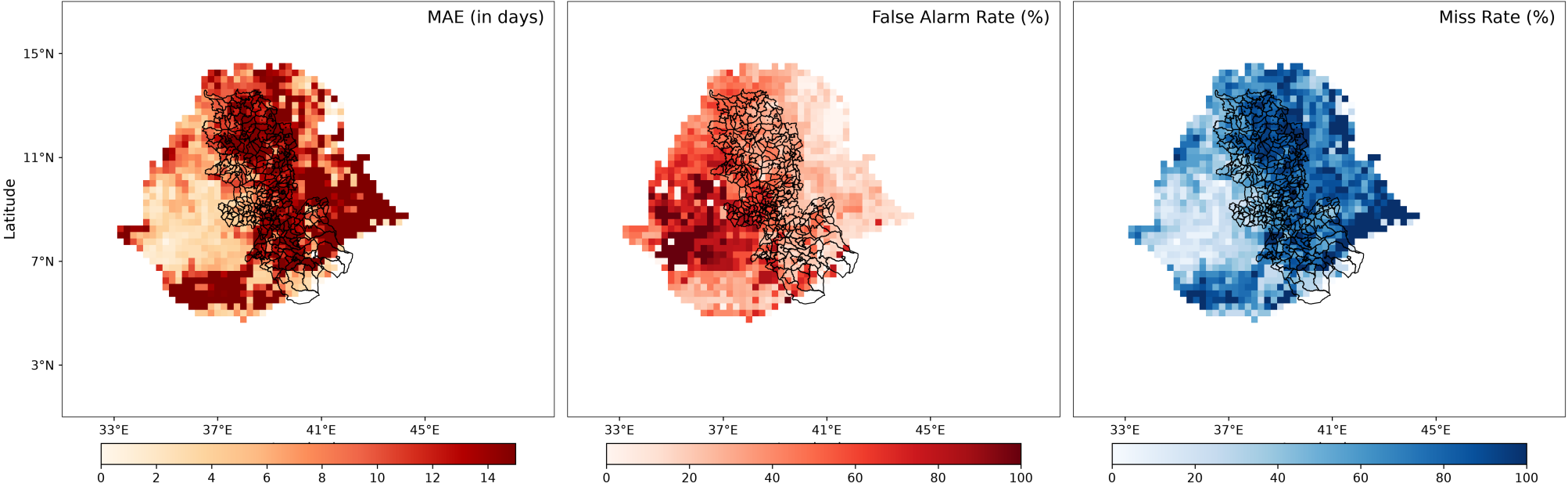
Spatial Metrics: Climatology (Days 1-15)
