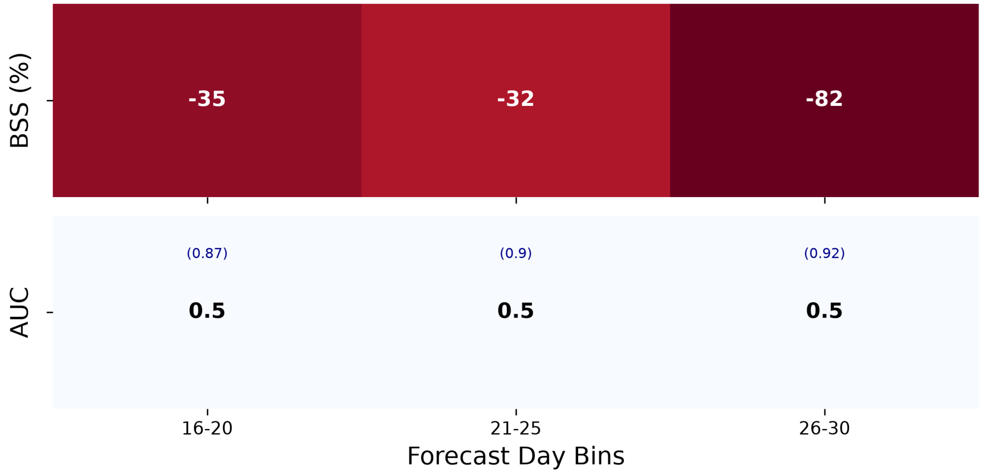
Skill Scores Heatmap - AIFS Ensemble - Days 16-30
