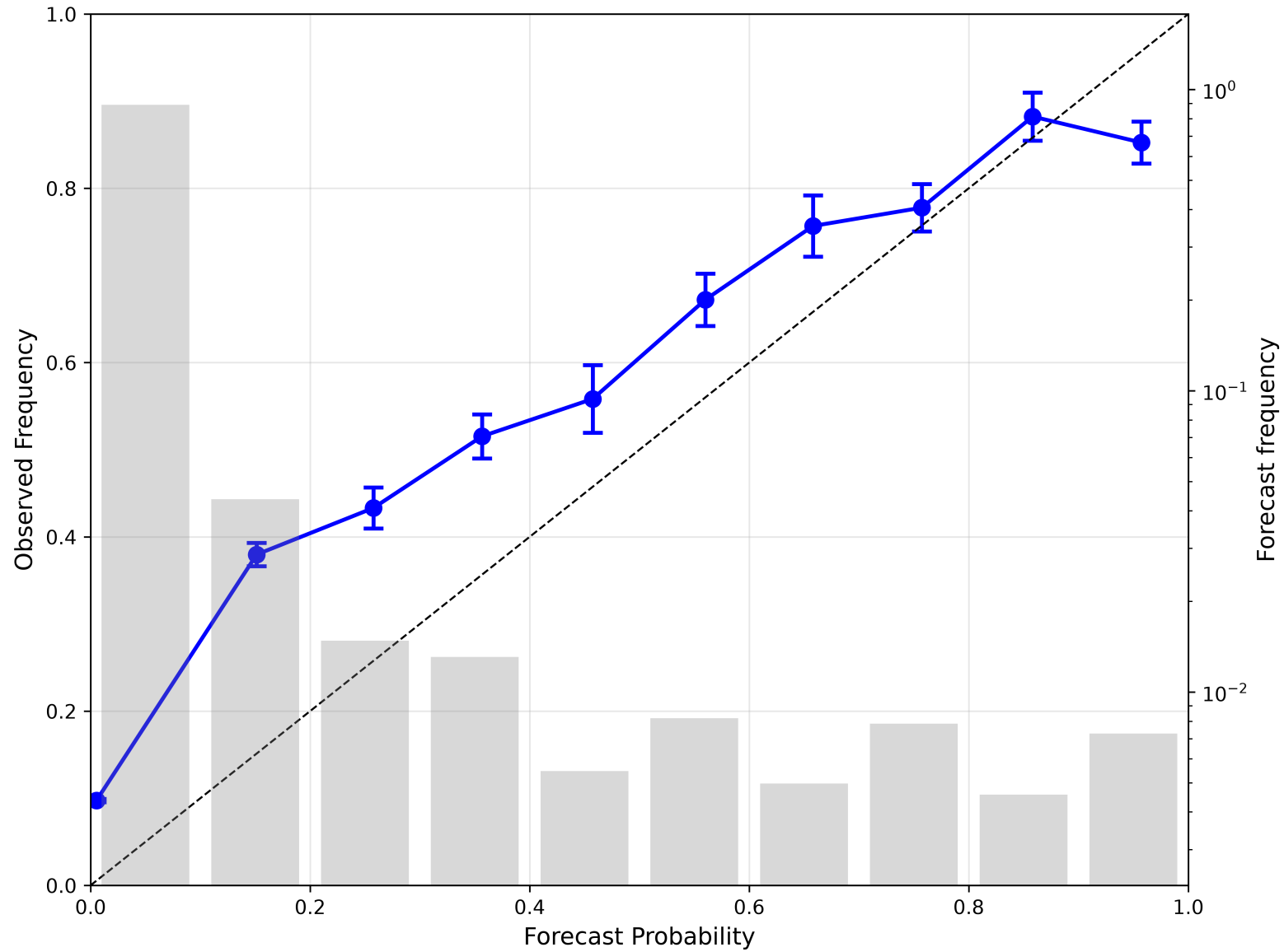
Reliability Diagram - AIFS Ensemble - Days 1-15
