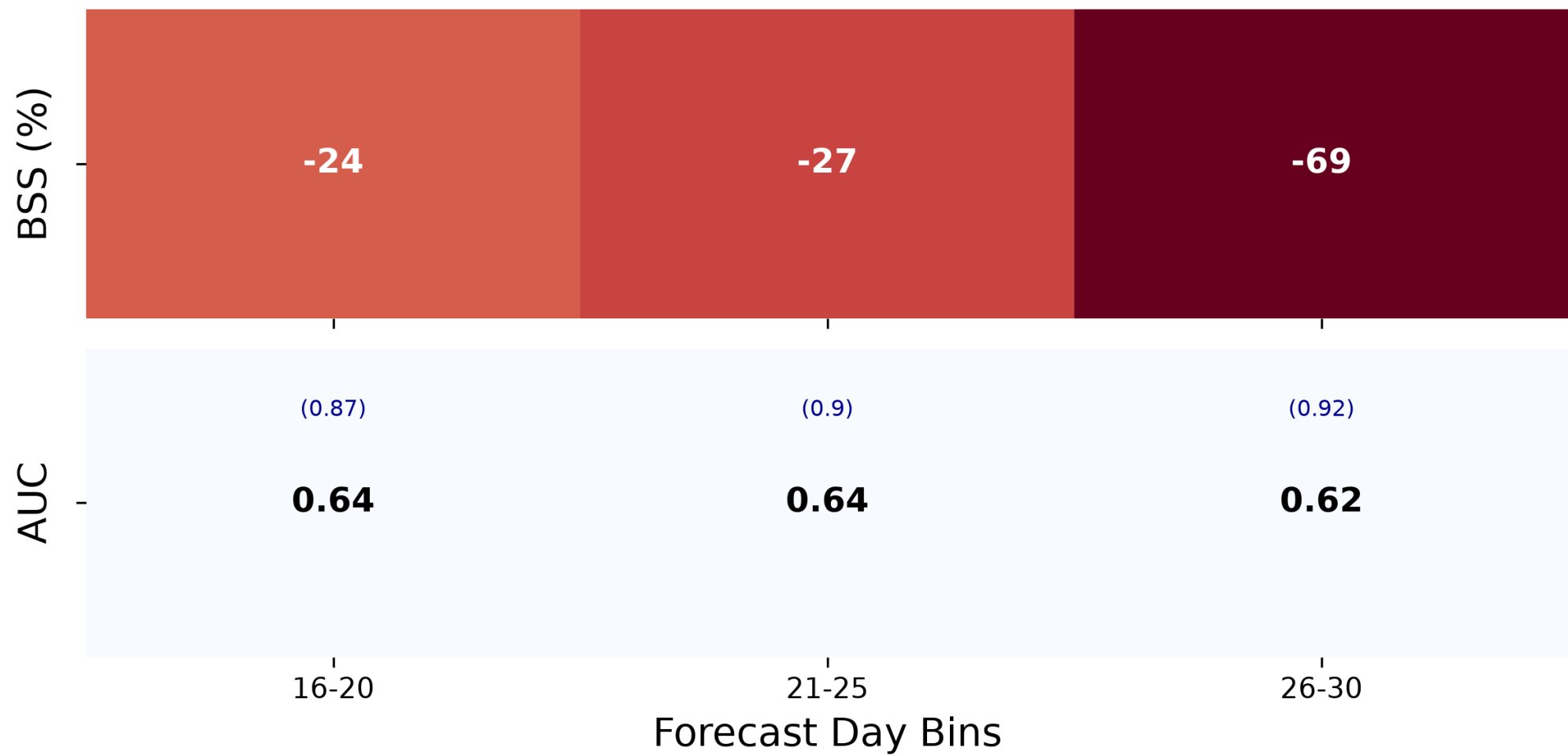
Skill Scores Heatmap - GenCast - Days 16-30
