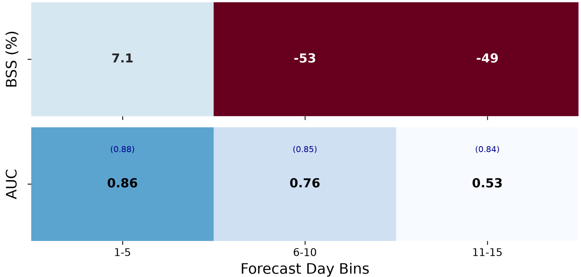
Skill Scores Heatmap - AIFS Ensemble - Days 1-15
