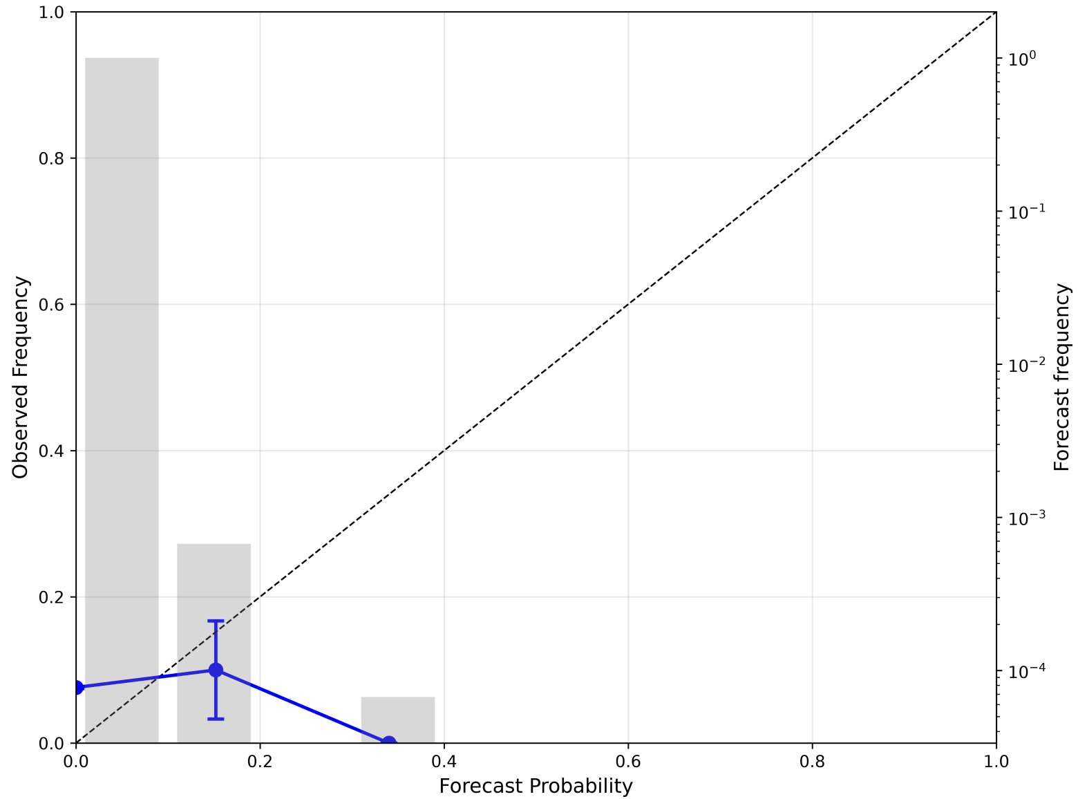
Reliability Diagram - AIFS Ensemble - Days 16-30
