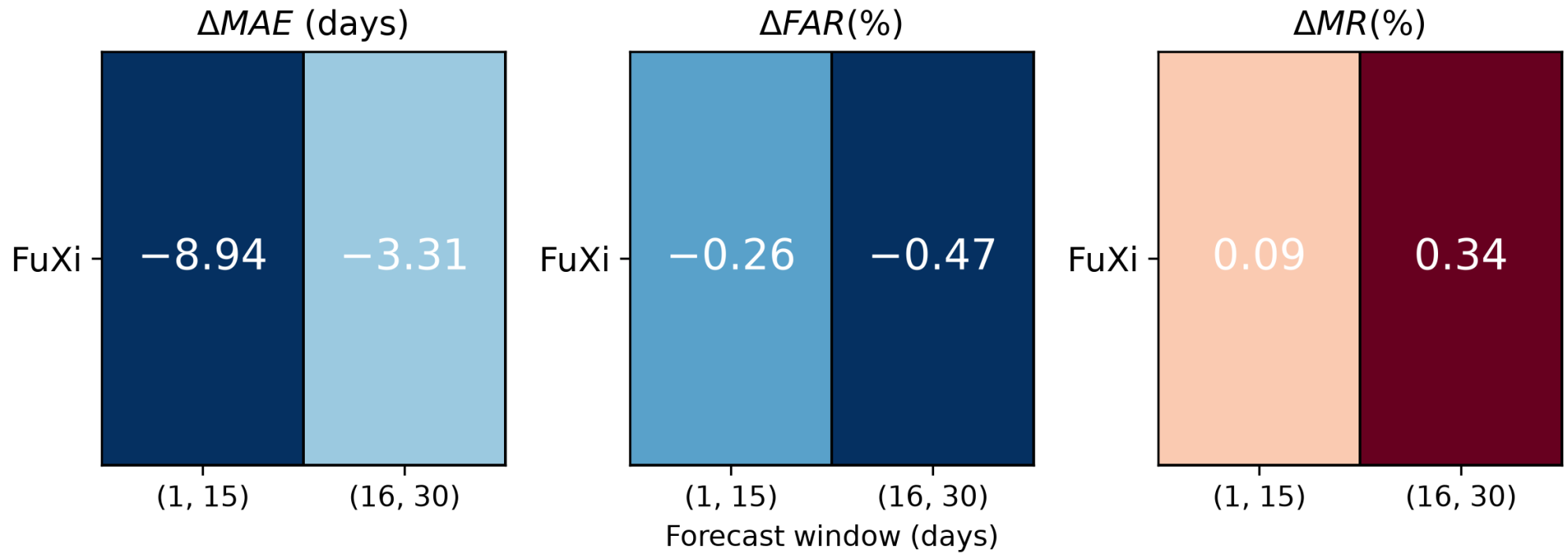
Panel Portrait MAE / FAR / MR - FuXi - 30-day
