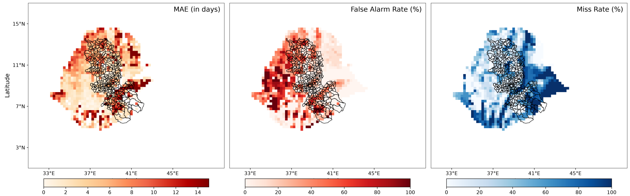
Spatial Metrics - GraphCast - Days 1-15
