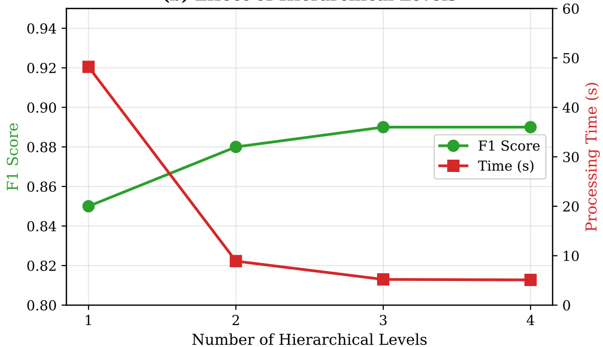
(b) Effect of Hierarchical Levels
