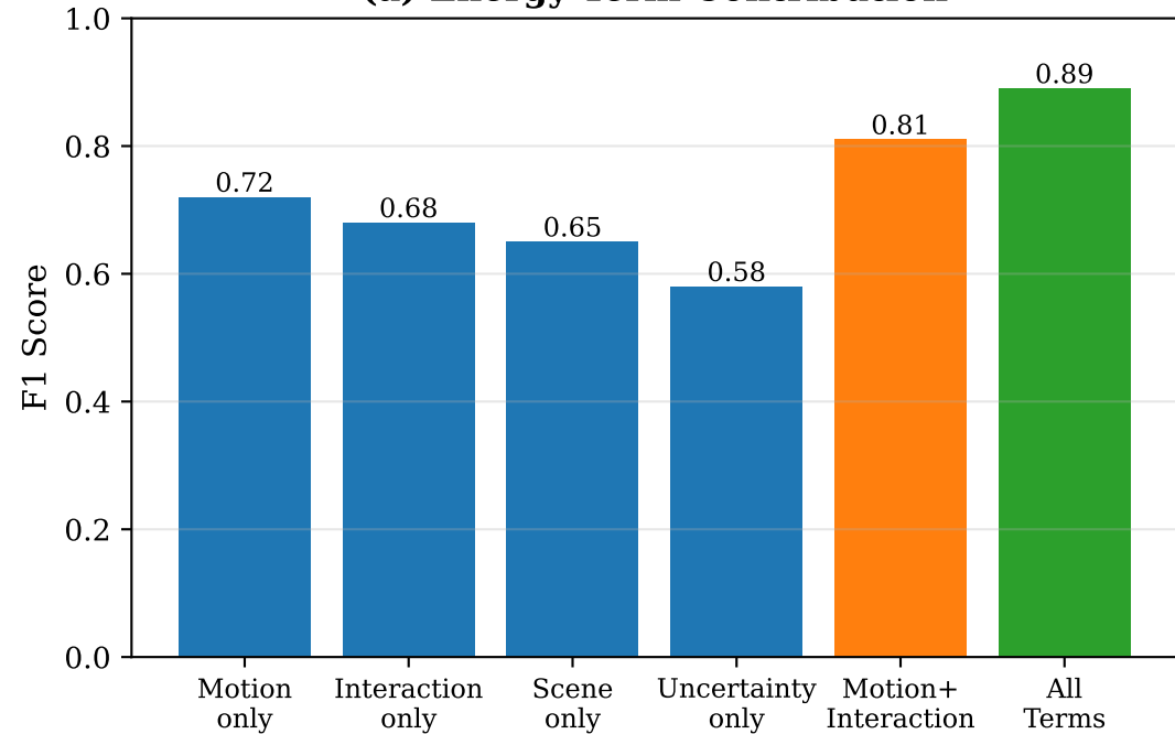
(a) Energy Term Contribution
