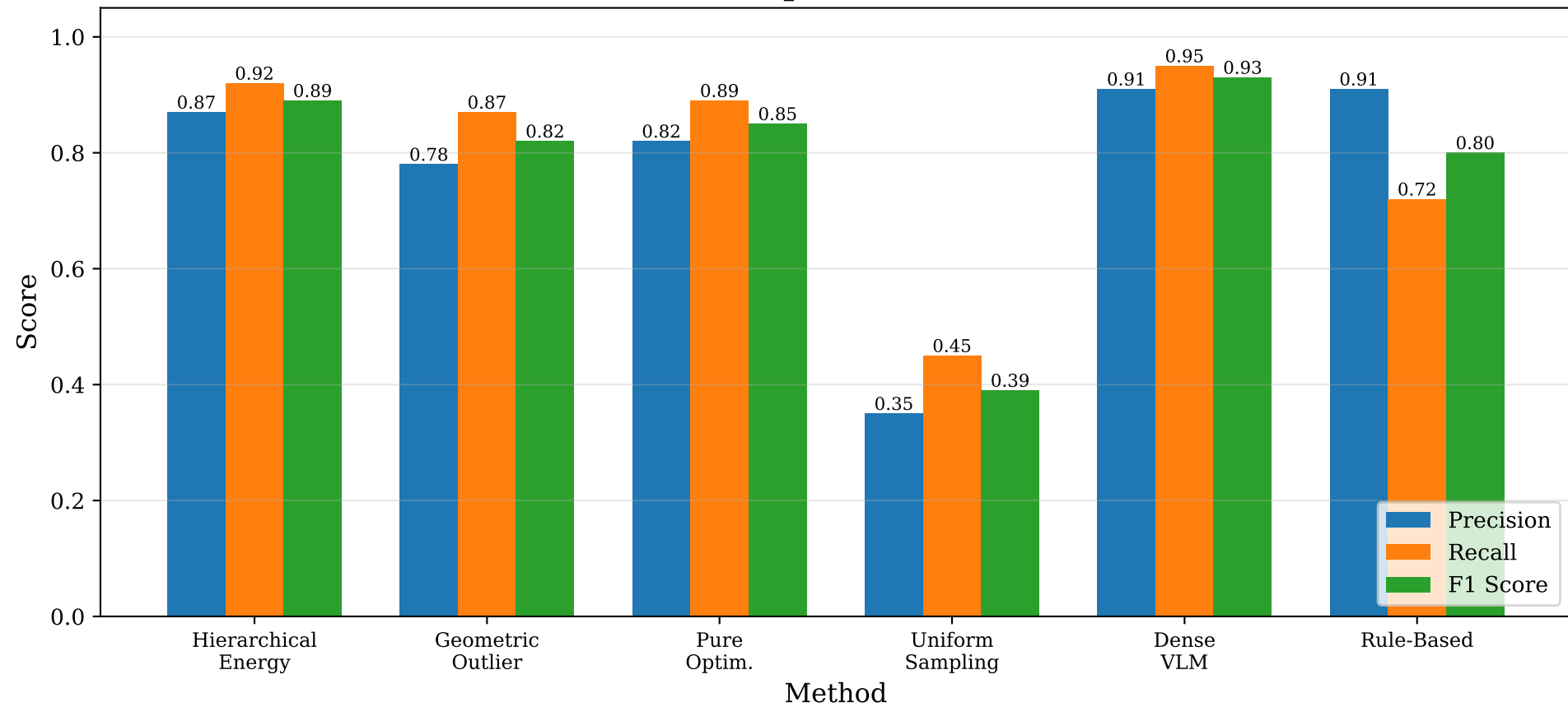
Performance Comparison Across Methods
