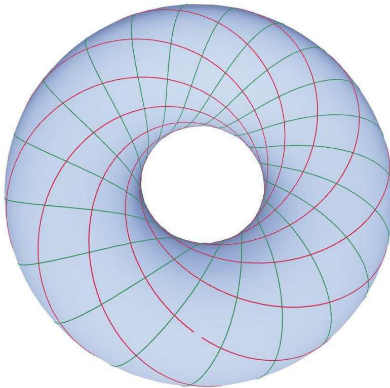
(图 36: 超结构化四边形网格, Geometric 软件作图。) (Figure 36: Super Structured Quad Mesh, generated by Geometric.)
