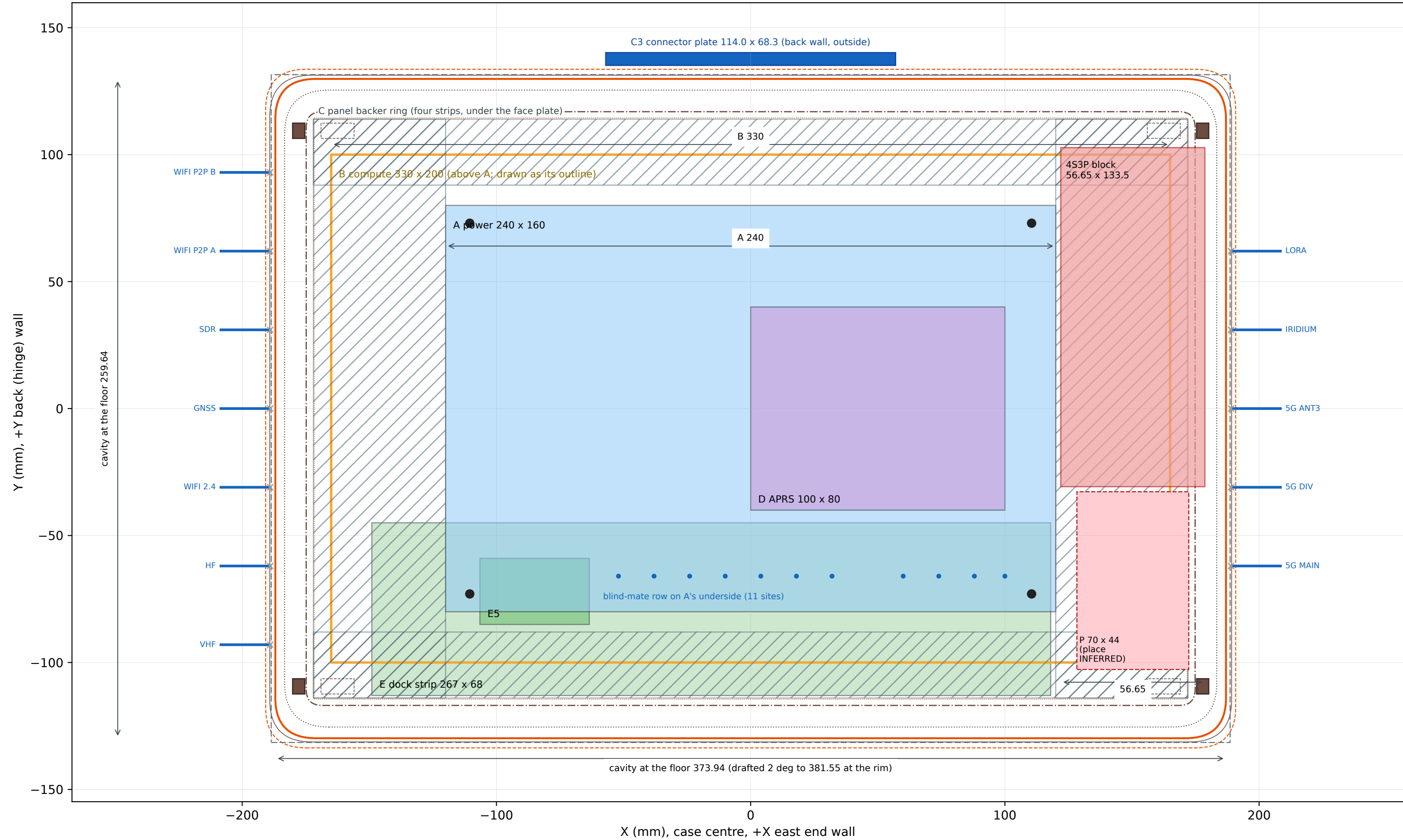
Case interior, plan view: Peli 1450 with the 1450PF frame, the board set and the pack (design drawing of an unbuilt prototype)
