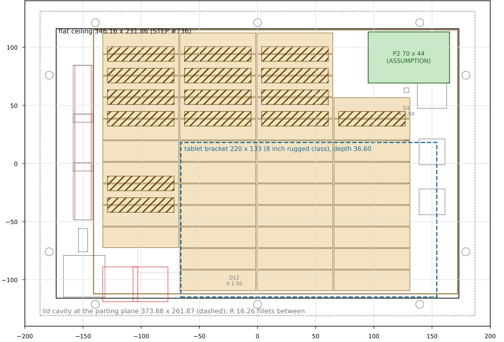
C: 8 inch tablet kept, HF out of the lid 58 cells: 4S14P in the lid, 4S20P with the base
