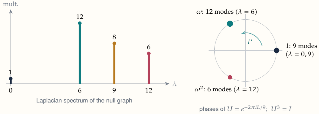
Figure 7. Left: the four Laplacian frequencies of the null graph. Right: running the graph as a quantum walk for time 2\pi/9 sends every mode to a cube root of unity — the 27-event present carries an exact qutrit-valued clock.
