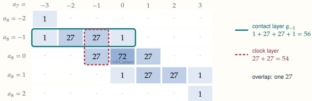
Figure 17. The 240 roots of E_8 counted by contact degree a_8 (rows) and clock degree a_7 (columns). The Freudenthal 56 (solid outline) and the clock’s first-order 54 (dashed outline) share exactly one 27.
