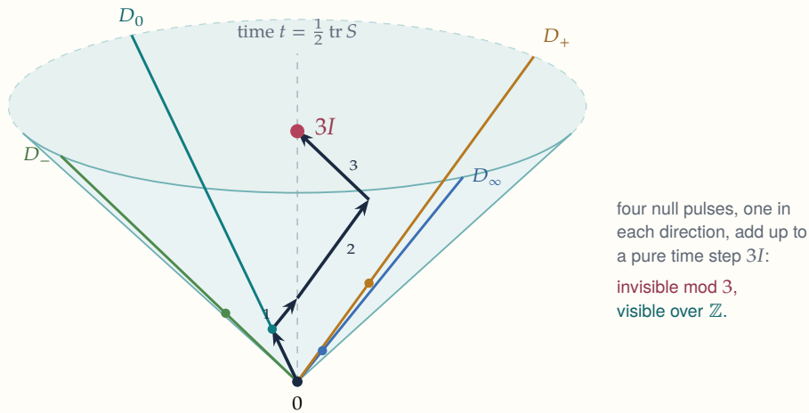
Figure 6. The real light cone of 2 \times 2 symmetric matrices, drawn with time t = \frac{1}{2} \text{tr } S upward. The four null rays D_0, D_\infty, D_+, D_- are the lifts of the four points of the Bell line. The black zig-zag adds one pulse in each direction: it ends on the time axis at 3I . Modulo three this is the zero matrix — the finite present cannot see it — but the integer lift records it as elapsed proper time.
