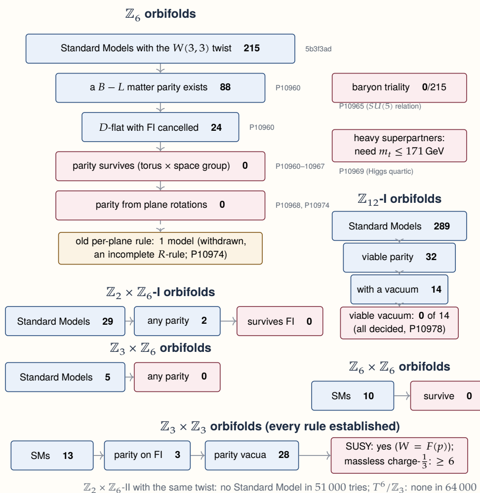
Figure 28. The vacuum gauntlet. Blue: filters passed; red: dead ends; gold: a door that looked open and was withdrawn. The last row is the one family where the parity survives: its vacua are supersymmetric, and a hidden-representation index leaves six massless charge- \frac{1}{3} states in each (P10979, P11024). Every count is exact (Farkas certificates, Smith normal forms, lattice tests and integer programs), and each is regenerated by the script named in the ledger.
