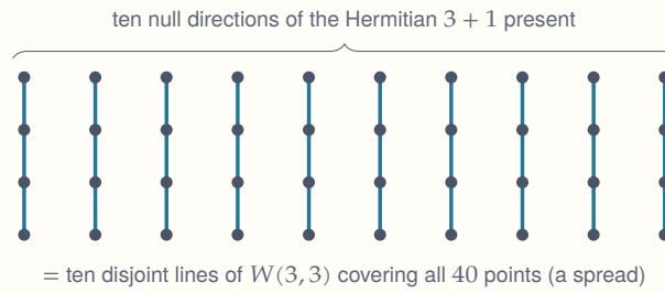
Figure 11. The Hermitian 3 + 1 light cone is a partition of the forty points into ten complete measurement contexts — a complete “schedule” for measuring every two-qutrit direction exactly once.
