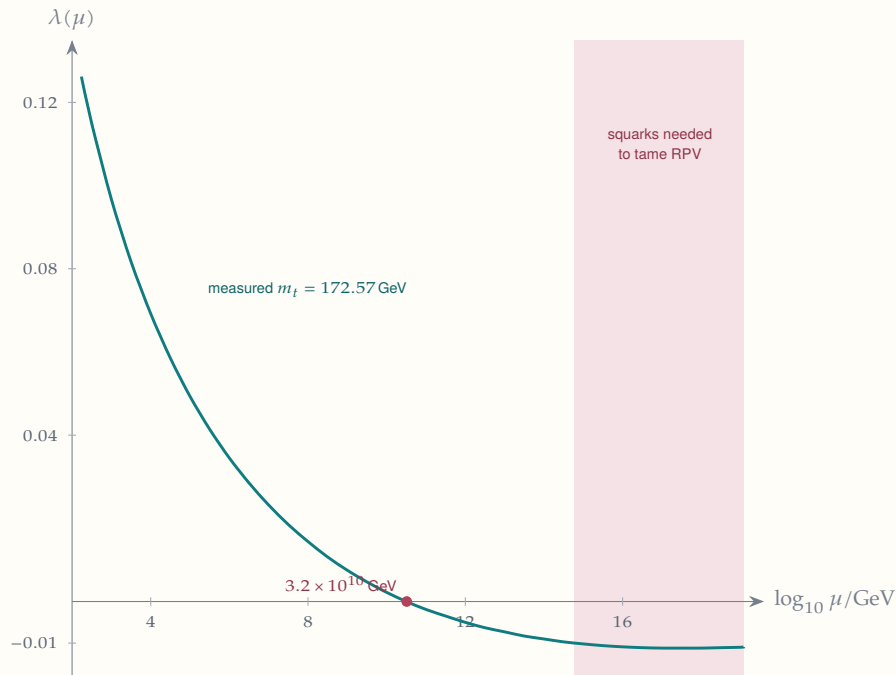
Figure 32. The Higgs self-coupling run to high energy (two loops, NNLO matching). It turns negative near 3 \times 10^{10} \text{ GeV} , far below the \gtrsim 6 \times 10^{14} \text{ GeV} that heavy squarks would need to make the regenerated R -parity violation harmless (shaded).
