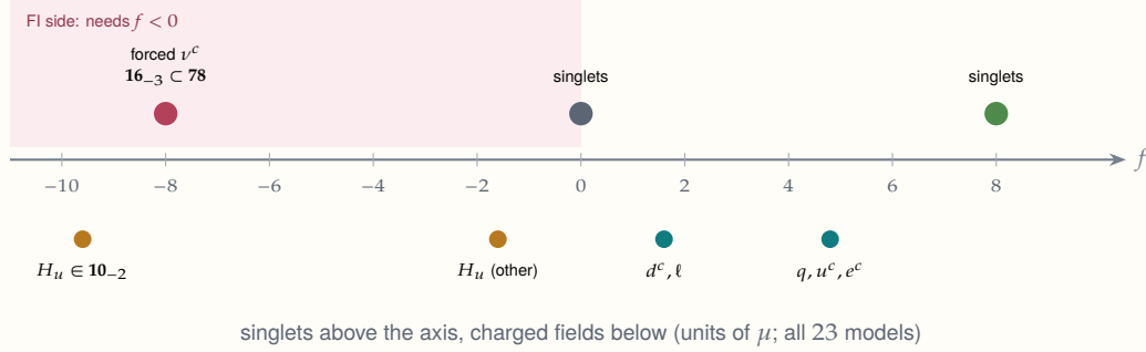
Figure 30. The canonical certificate f = 4Q_\psi - \frac{4}{5}Q_\chi on the families. Among singlets, only the right-handed-sneutrino direction of the E_6 adjoint's \mathbf{16}_{-3} sits on the side that can balance the Fayet–Iliopoulos term.
