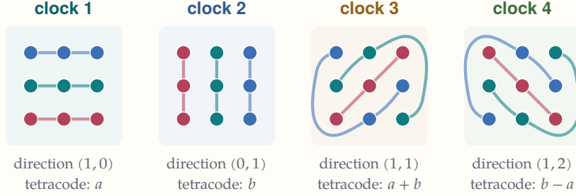
Figure 9. The four Hesse clocks. Each panel shows the nine operator histories of one qutrit as the affine plane \mathbb{F}_3^2 , split into three parallel lines (the three “ticks”). Lines of the two diagonal classes wrap around, as on a torus. The four panels are labelled by the four points of \mathbb{P}^1(\mathbb{F}_3) — the same four labels as the null directions of Figure 4 — and by the coordinate of the tetracode they read.
