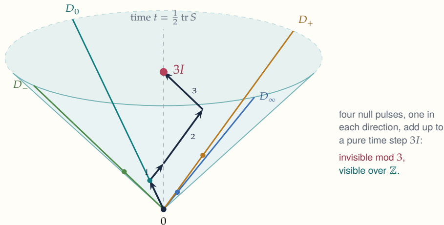
Figure 6. The real light cone of 2 \times 2 symmetric matrices, drawn with time t = \frac{1}{2} \text{tr } S upward. The four null rays D_0, D_\infty, D_+, D_- are the lifts of the four points of the Bell line. The black zig-zag adds one pulse in each direction: it ends on the time axis at 3I . Modulo three this is the zero matrix — the finite present cannot see it — but the integer lift records it as elapsed proper time.
