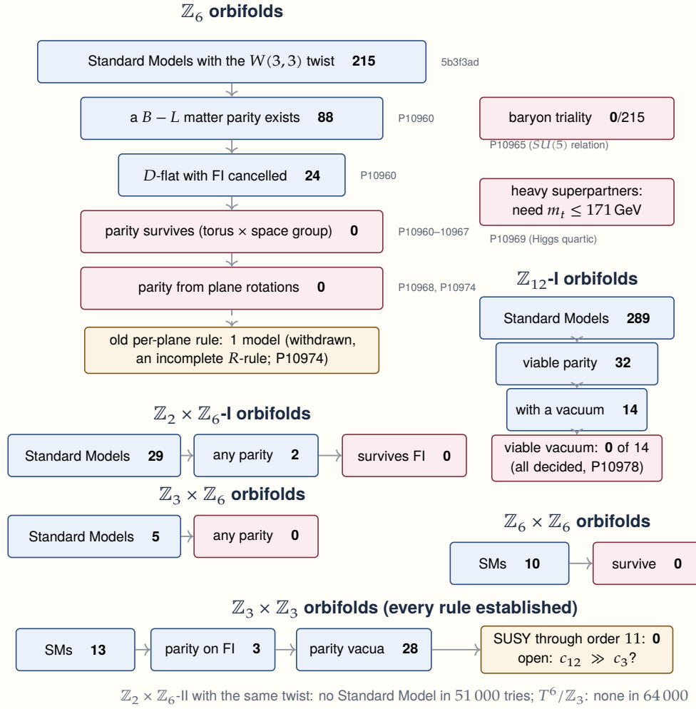
Figure 28. The vacuum gauntlet. Blue: filters passed; red: dead ends; gold: a door that looked open and was withdrawn (left), and the one that is still open, stated as a coupling inequality (bottom right). Every count is exact (Farkas certificates, Smith normal forms, lattice tests and integer programs), and each is regenerated by the script named in the ledger.
