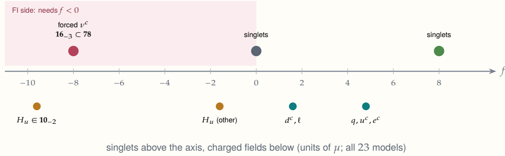
Figure 30. The canonical certificate f = 4Q_\psi - \frac{4}{5}Q_\chi on the families. Among singlets, only the right-handed-sneutrino direction of the E_6 adjoint's \mathbf{16}_{-3} sits on the side that can balance the Fayet–Iliopoulos term.
