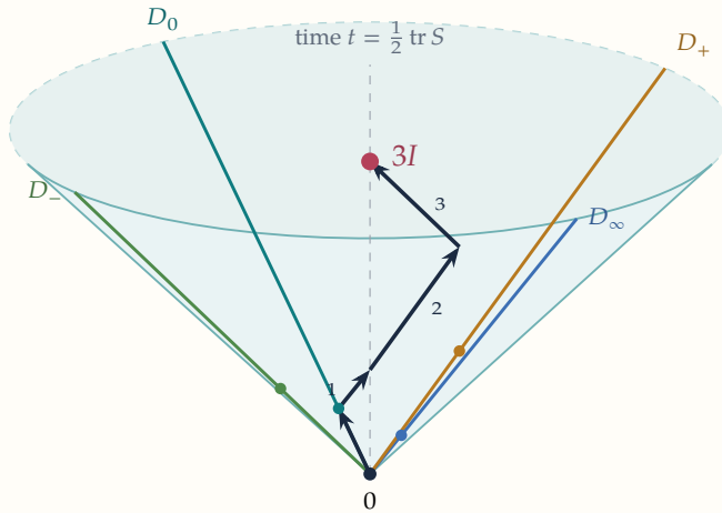
Figure 6. The real light cone of 2 \times 2 symmetric matrices, drawn with time t = \frac{1}{2} \text{tr } S upward. The four null rays D_0, D_\infty, D_\pm are the lifts of the four points of the Bell line. The black zig-zag adds one pulse in each direction: it ends on the time axis at 3I . Modulo three this is the zero matrix — the finite present cannot see it — but the integer lift records it as elapsed proper time.
