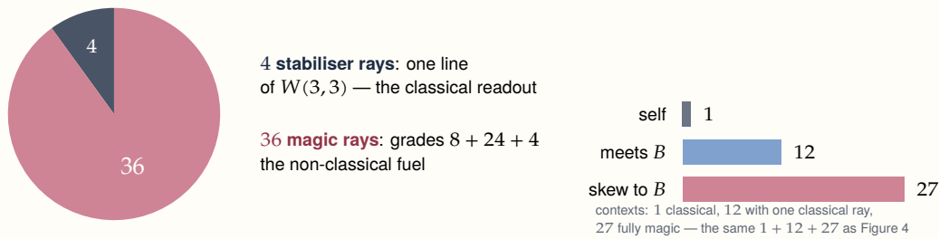
Figure 35. The machine’s quantum resource is the geometry itself: remove one line and every remaining point is a magic state.
