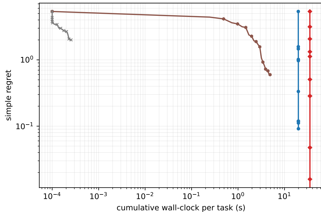
cold start (pre-training charged to one task)
