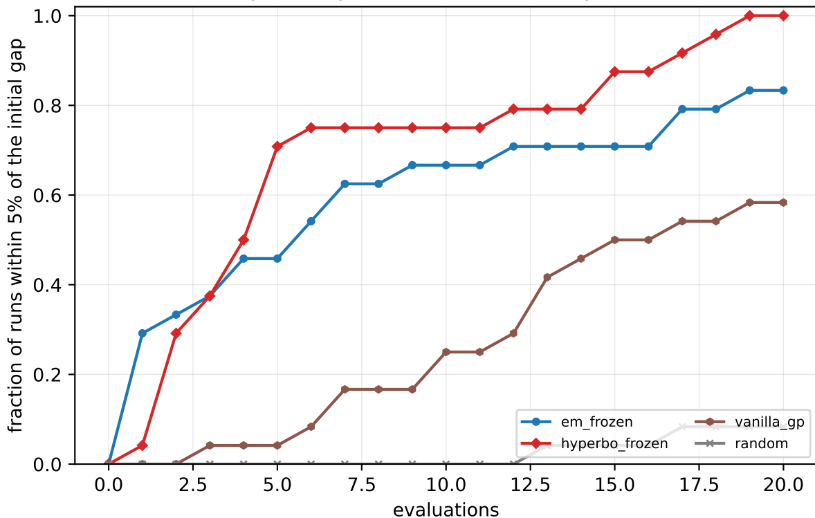
Batch BO q=1 (sequential control): data profile (tol=5%)
