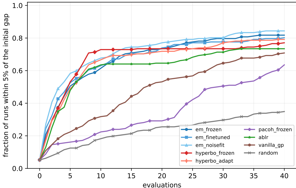
LCBench 7D BO (12 datasets x 16 seeds): data profile (tol=5%)
