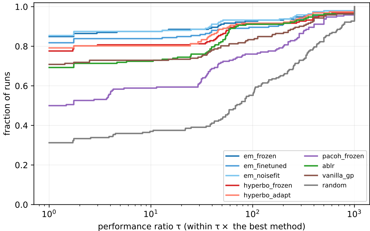
LCBench 7D BO (12 datasets x 16 seeds): performance profile (final regression)
