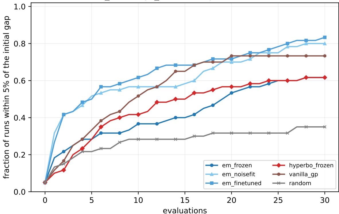
ood_shrinkage_a0.0: data profile (tol=5%)
