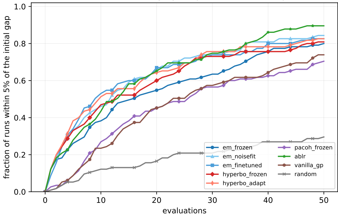
PD1 full: LOO over 23 tasks, neglog warp (115 runs): data profile (tol=5%
