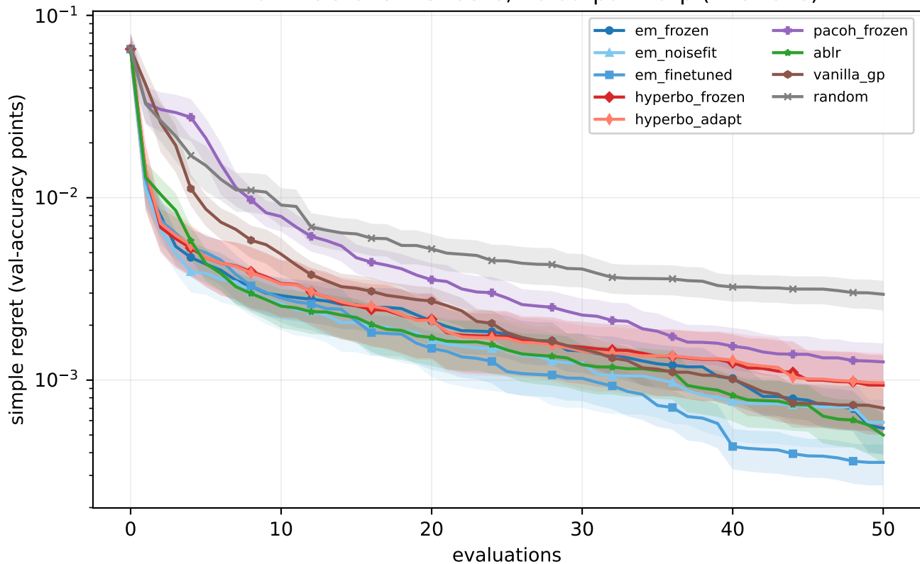
PD1 full: LOO over 23 tasks, no output warp (115 runs)
